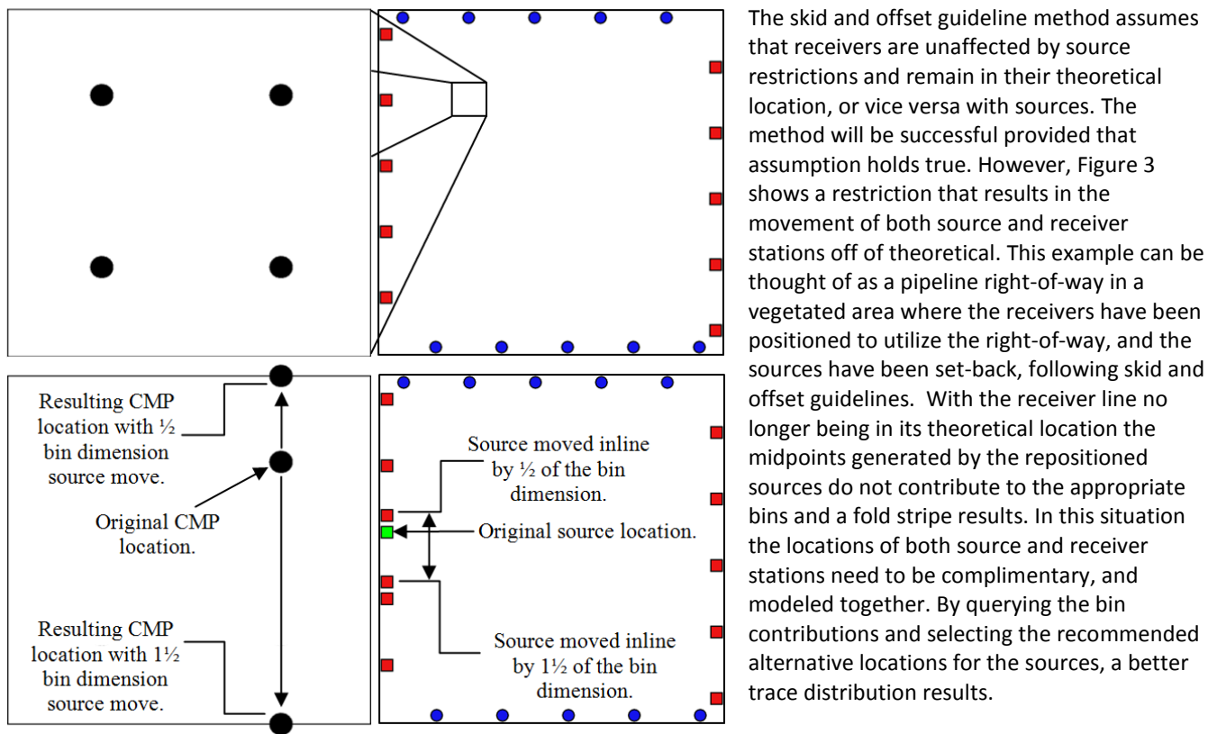
Figure 2: Top-right panel – Double stagger layout, sources are coloured red, receivers blue. Top-left panel – blown up view of a bin grid showing organized CMP scatter. Bottom-right – movement of one particular source North \frac{1}{2} a bin grid dimension, and also South by 1\frac{1}{2} a bin grid dimension. Bottom-left – CMP location from source movements are now located at the bin edge.
