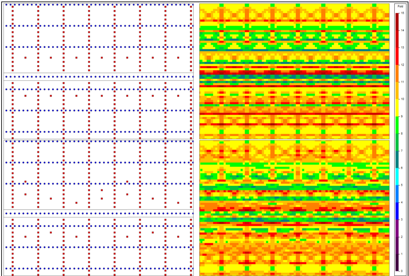
Figure 3: Top-left panel – an East-West receiver line has been offset off of its theoretical location, and sources have followed typical skid and offset guidelines. Top-right panel, the resulting fold from the movements in the top-left panel. Bottom-left panel – the receiver line has moved, but sources have now been positioned using the optimal restriction modeling method. Bottom-right panel – the fold that results from the movements in the bottom-left panel.
