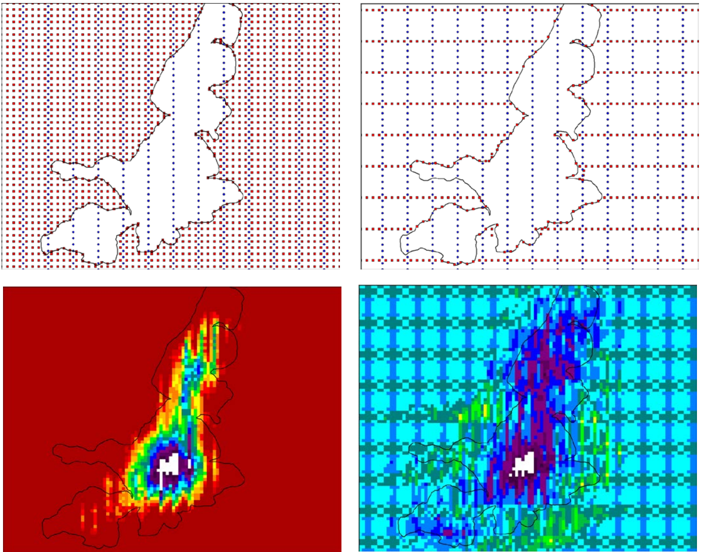
Figure 4: Top-Left Panel – Every available “full wavefield” location for a source outside of a restriction is being used. Top-Right Panel – optimal restriction model layout for a given set of attribute constraints. Bottom-Left Panel – fold plot from top panel layout. Bottom-Right Panel – fold plot from optimal restriction model layout. Note that zero fold bins are now filled and a more even trace distribution across the restriction.
